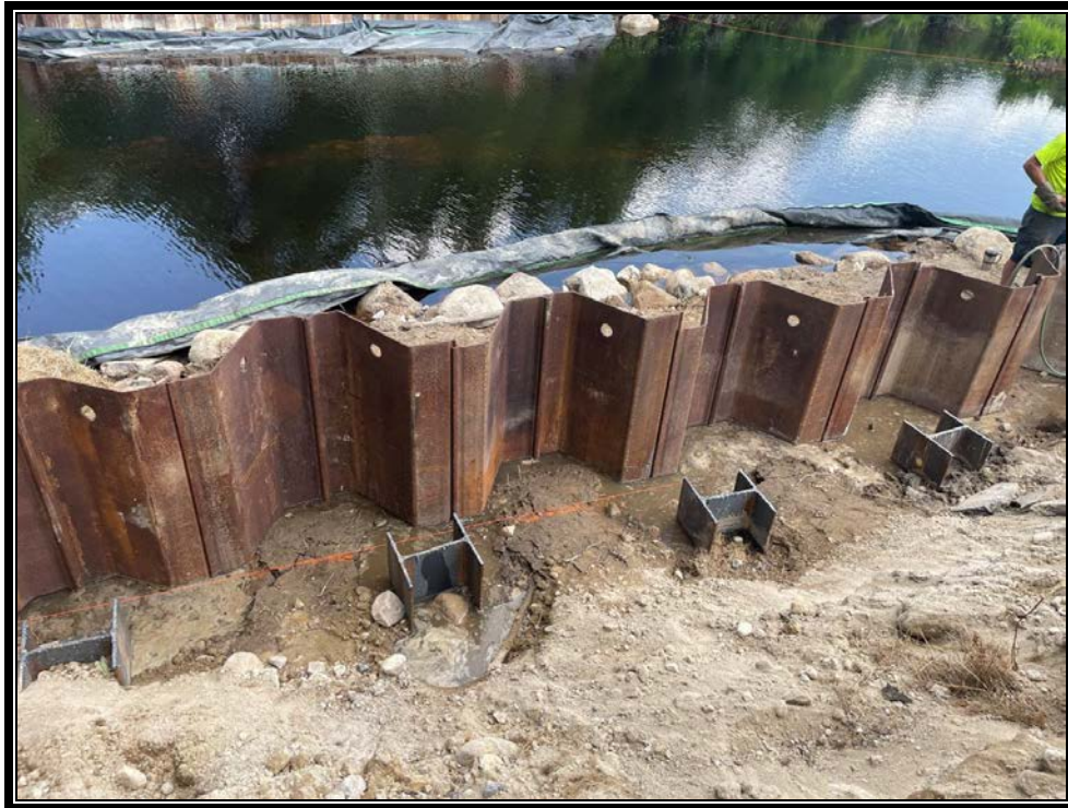
Photo 2: Sheet pile installed.
