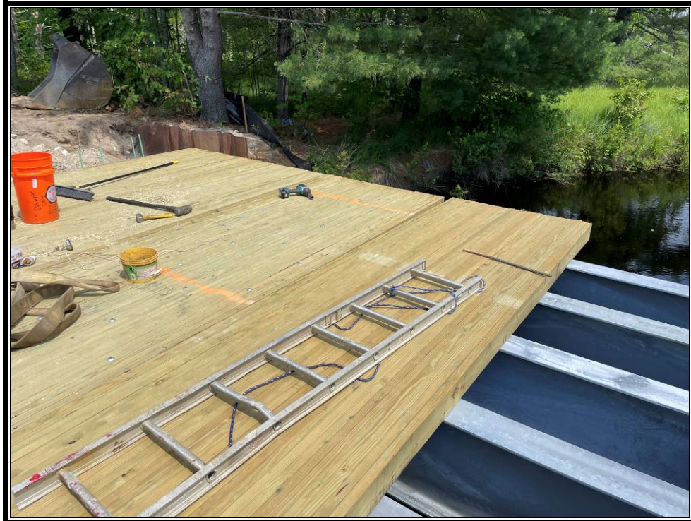
Photo 1: Deck section number 3 placed into position.
