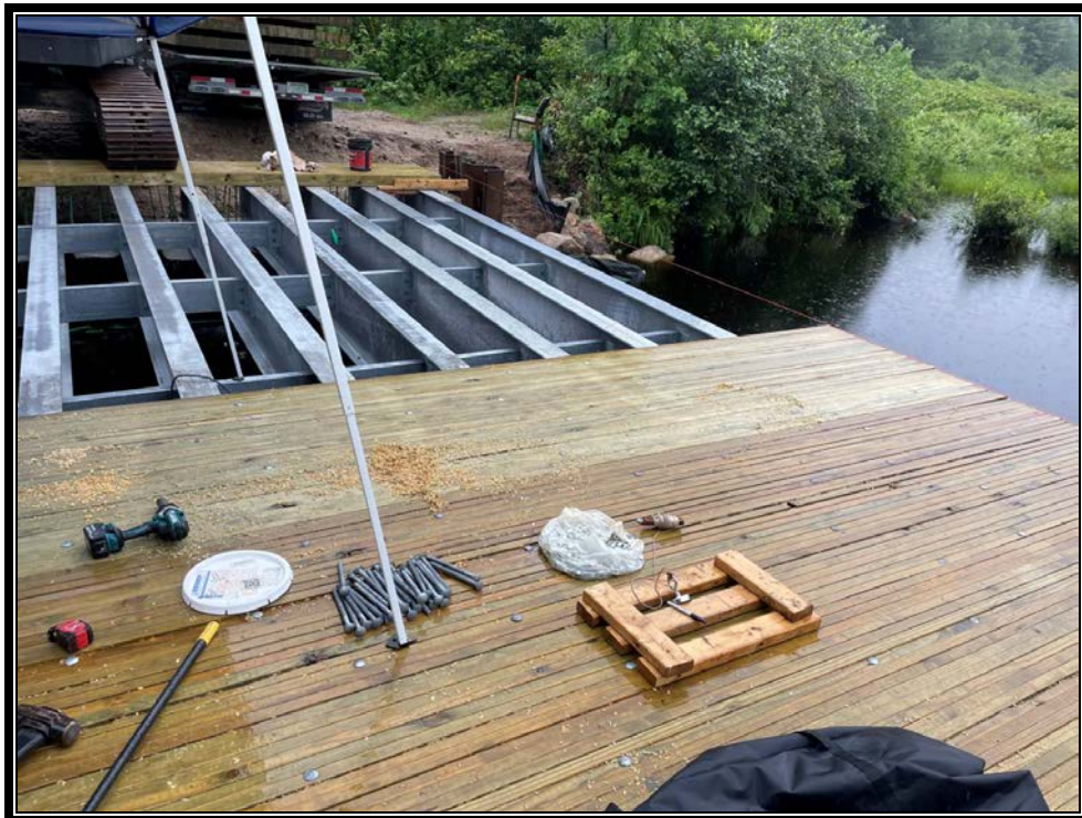
Photo 1: Deck section number 6 placed into position.
